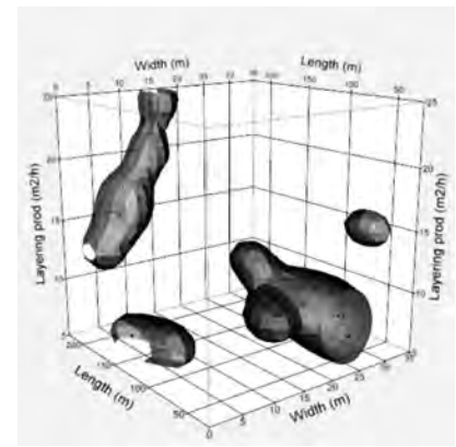
Figure 3: Scatterplot 3D graph for trivariate outliers detection.
